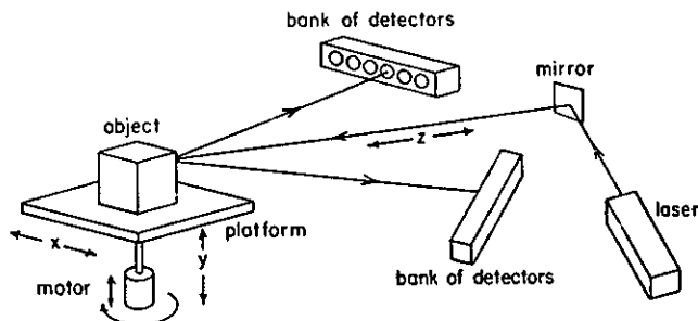
Fig. 2. Laser ranging system.
