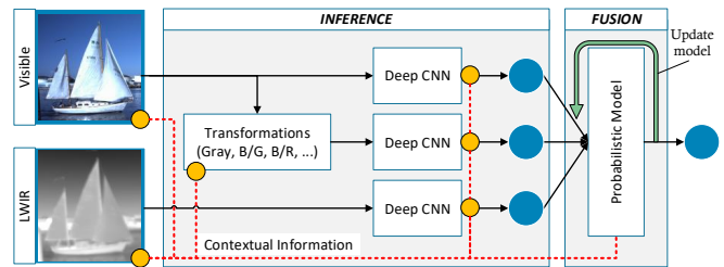
Fig. 1: Overview of DyFusion. The inference receives data from sensors and outputs probabilities over vessel labels. The fusion updates the sensor probabilities using contextual data.
