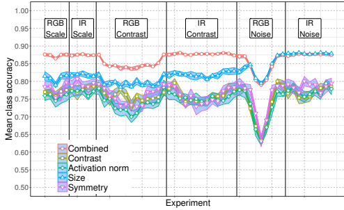
Fig. 3: DyFusion accuracy per contextual variable.
