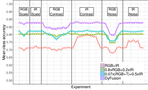
Fig. 2: DyFusion and baseline accuracy in different experiments.
