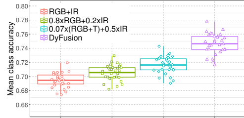
Fig. 4: Mean class accuracy for 54 experiments where random scale, SNR and contrast values are applied to test samples.
