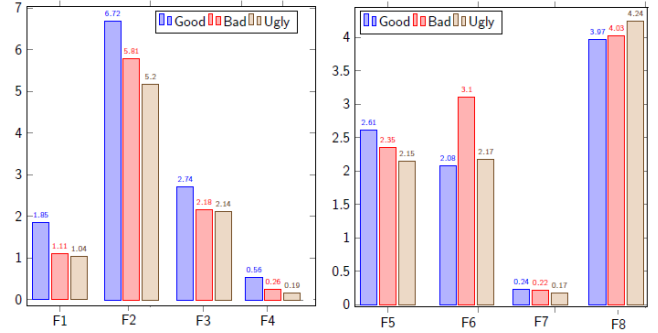
Figure 4. Gabor features used to train the multi-class perceptron classifier for image patch quality assessment. The features were computed from the kurtosis and skewness of the Gabor filter responses of the image patches. F1 and F4 are the peak and mean skewness of the magnitude response, respectively. F2 and F5 are the peak and mean kurtosis of the phase response, respectively. F3 is the mean kurtosis of the magnitude response. F6 and F7 are the peak and mean skewness of phase response, and F8 is the peak of the magnitude response. F7 was scaled up by 0.2 for visibility. The charts show that together, the features exhibit discriminative potential for classifying patches into good, bad and ugly bins.
